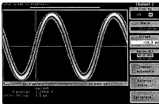
Agilent 83434A recovered clock output at 9953.28 MHz*
