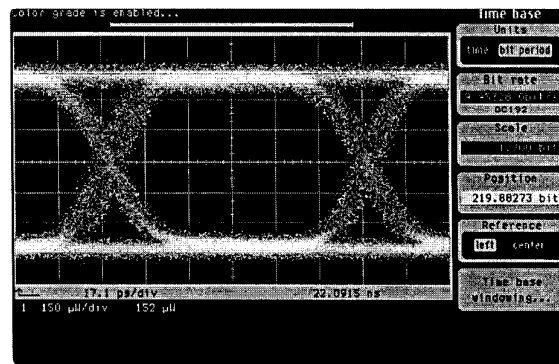
Agilent 83433A unfiltered optical waveform at 9953.28 Mb/s*
