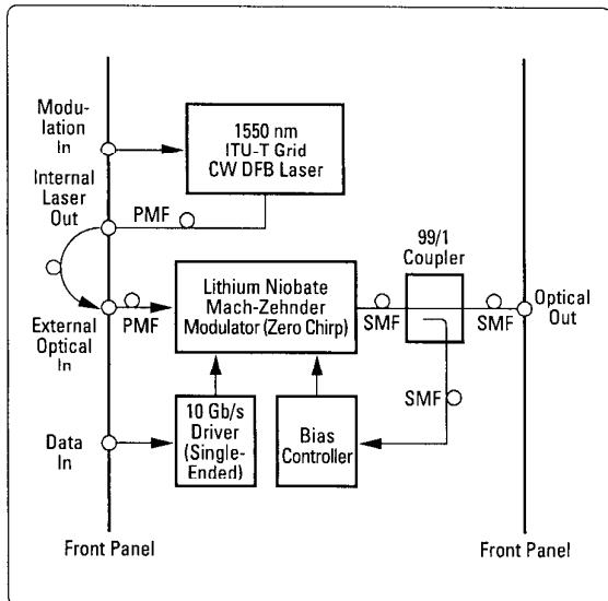
83433A block diagram
