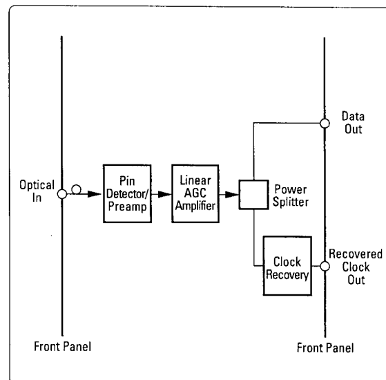
83434A block diagram
